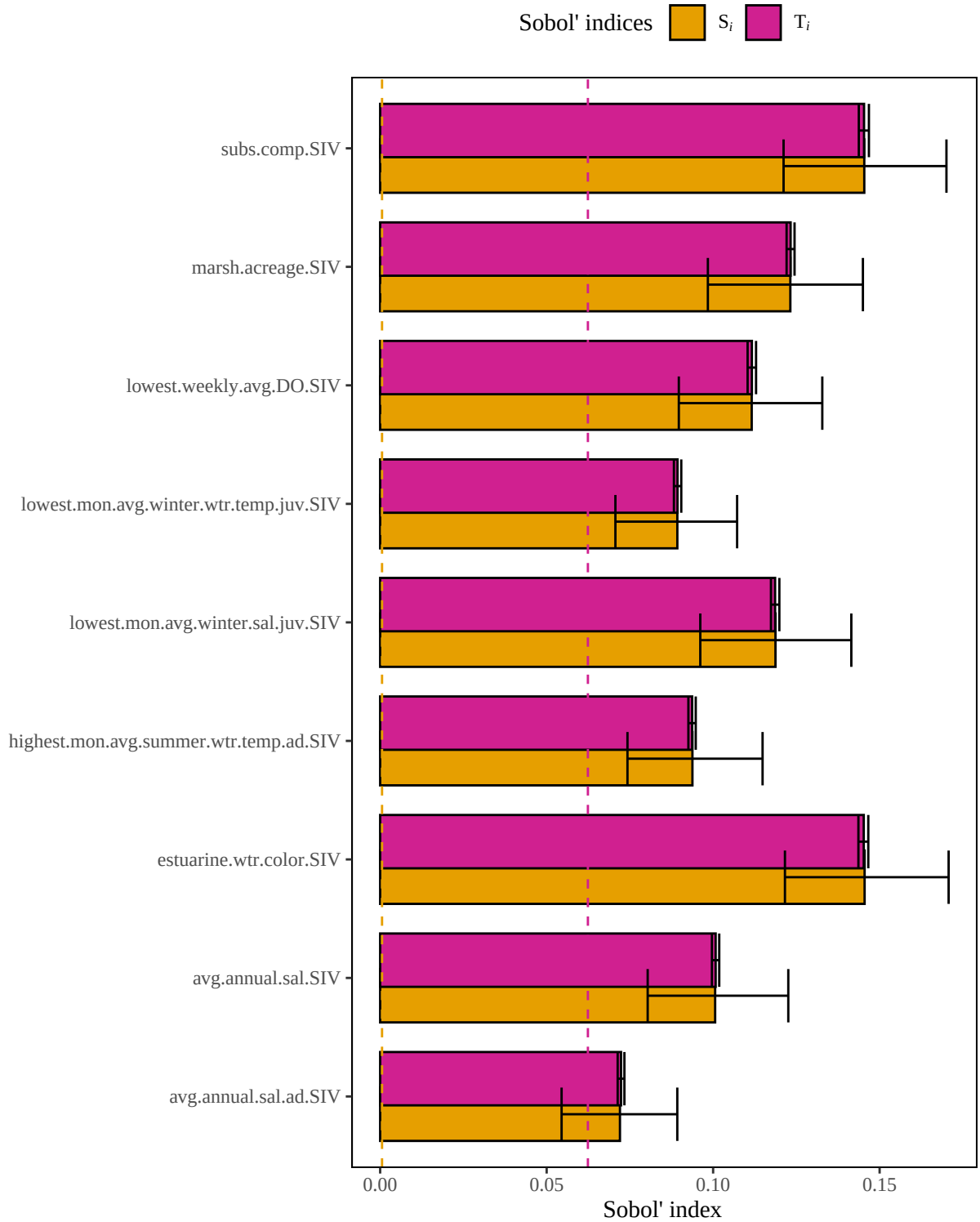
Figure 4. Results of a sensitivity analysis for the gulfmenhadenEstuary model based on an arithmetic mean structure. Dashed lines represent baseline numerical approximation error for S_i and T_i ( i.e. , dummy variables).
