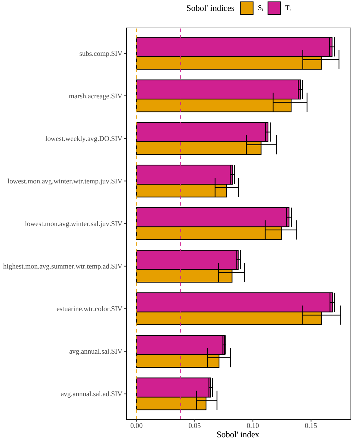
Figure 5. Results of a sensitivity analysis for the gulfmenhadenEstuary model based on a geometric mean structure. Dashed lines represent baseline numerical approximation error for S_i and T_i ( i.e. , dummy variables).
